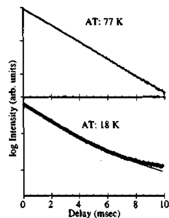
Figure 2. Phosphorescence decay of anthrone (AT) at 77 (top) and at 18 K (bottom) in methycyclohexane. The line on top and bottom traces correspond to the fits to single and double exponentials, respectively.
