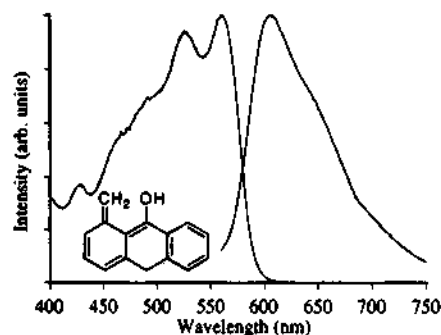
Figure 3. Excitation and emission spectra of the photoenol obtained upon irradiation of 1,4-DMAT in ethanol at 77 K.
